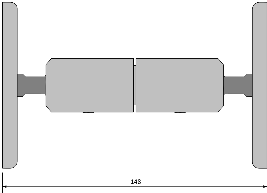
SE-DBLSVL mk II Installation Dimensions All Dimensions in millimeters
